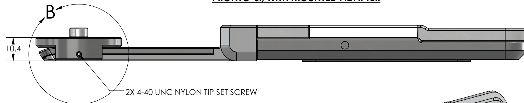
PRONTO-Si, WITH MOUNTED ADAPTER
