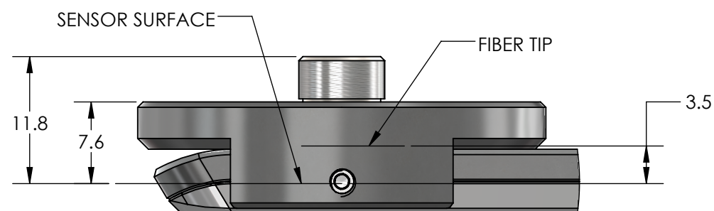
DETAIL B SCALE 2 : 1
