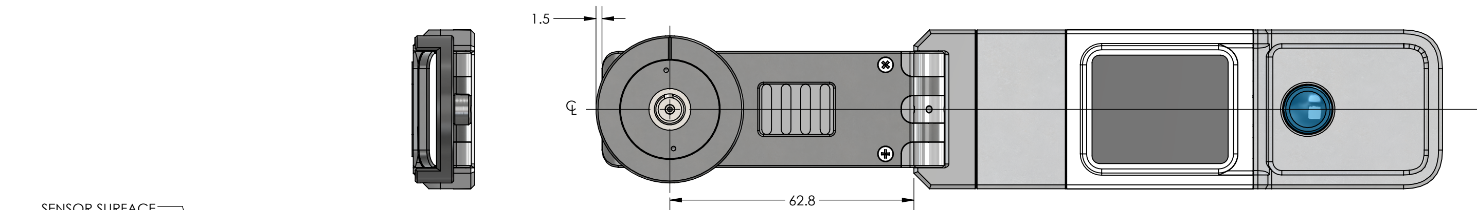
PRONTO-Si, WITH MOUNTED ADAPTER
