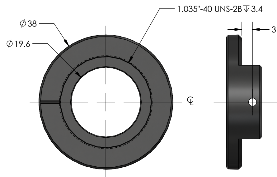
UNMOUNTED FILTER ADAPTER
