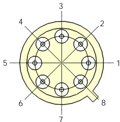
PINOUT TOP VIEW
