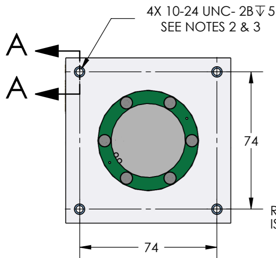
UP25N ASSEMBLY WITHOUT FRONT COVER
