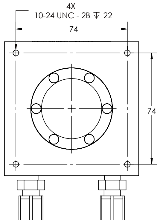
MOUNTING FROM FRONT WITHOUT COVER SEE NOTE 2
