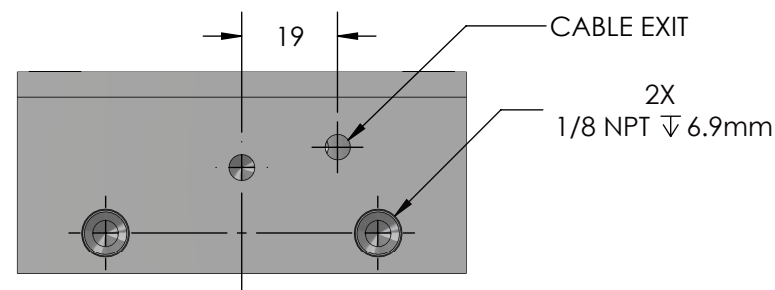
BOTTOM VIEW FITTINGS REMOVED
